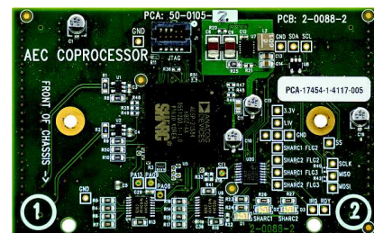
AEC Coprocessor
